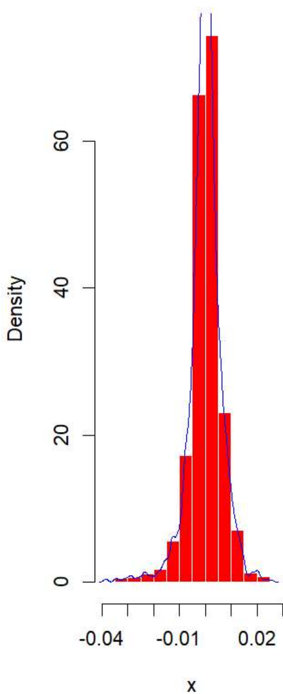
Histogram of x
